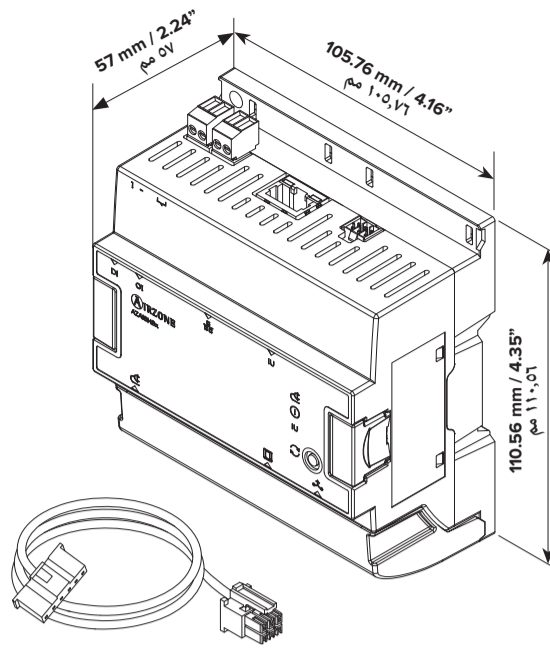
AZPV8WIRE17 2.5 m (8.2 ft) / 6x0.2 mm 2 2.5 m / 8.2 ft / 6x0.2 mm 2
