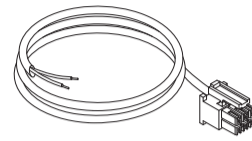
AZPV8WIRE10 2.5 m (8.2 ft) / 6x0.2 mm 2 2.5 m / 8.2 ft / 6x0.2 mm 2
