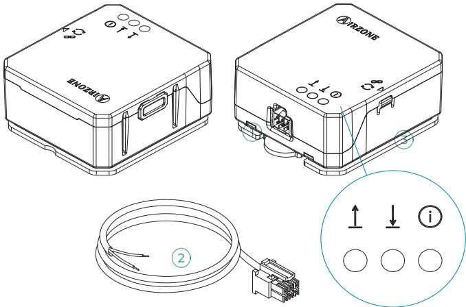
AZPV8WIRE10010 1 m / 6 x 0.2 mm²
