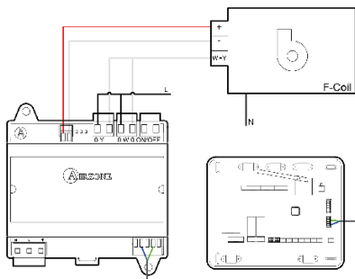
Instalace 2 trubek
