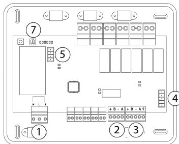
Radiant 3-4 tubes
