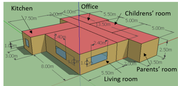
Figure 5. Floor plan of the home. 3D representation with measurements.
