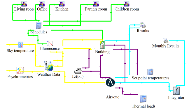
Figure 3. Setting up the zoned system in TRNSYS.
