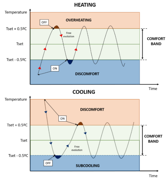
Figure 7. Evaluation of thermal comfort in a zoned system.
