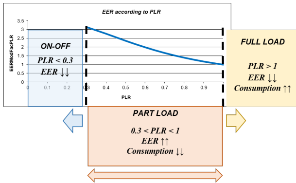
Figure 4. Diagram showing the different working regimes of an inverter unit.
